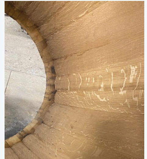
Noisette color of the inside of a DAMY barrel after the 2 hour super light long "Imperial" toast.
